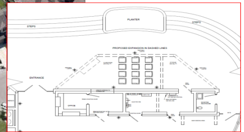
Pool Storage Building and expanded offices
